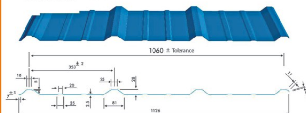
PLANNCO 1060 mm
